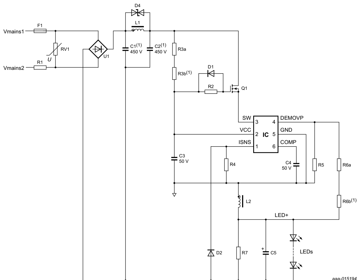
Fig 6. SSL5031CTS application diagram
